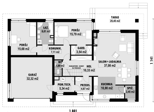
E-131 PARTER
