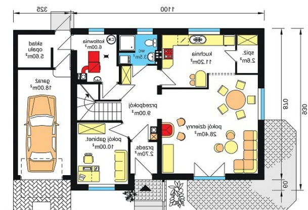
PARTER P-67.40m 2 , P-59.80m 2
