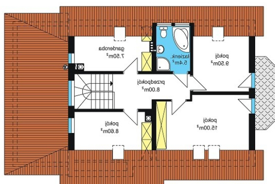
PODDASZE P-64.00m 2 , P-60.17m 2
